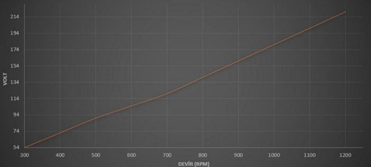
1500G-48V-Generator-Rpm-Volt-Graphic
