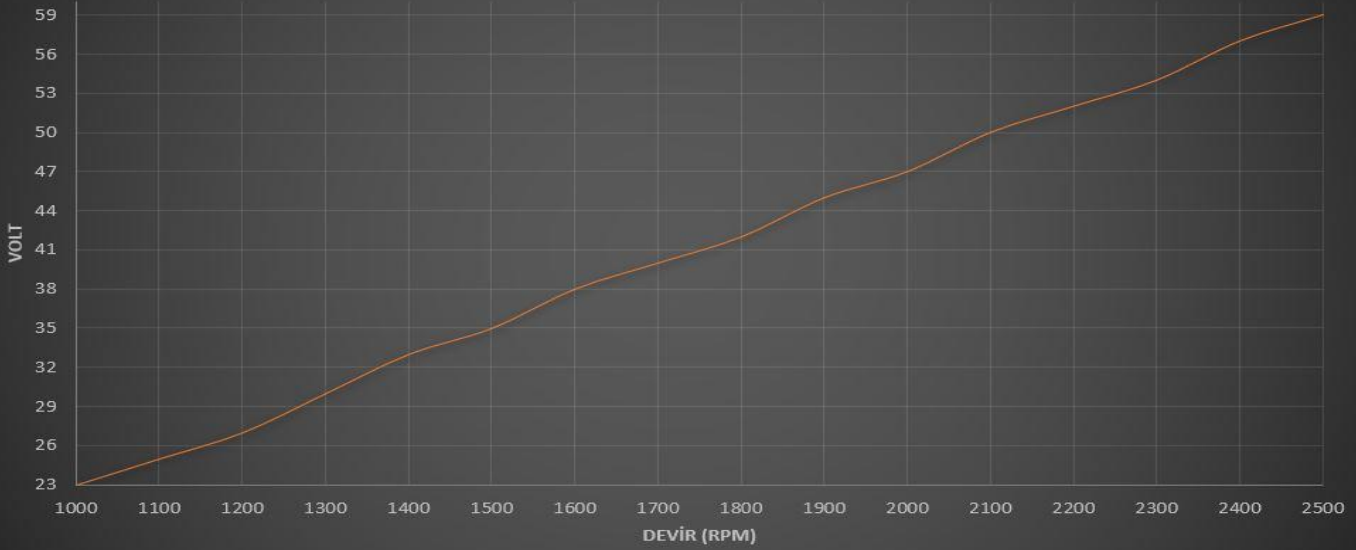
500G-12V-Generator-Rpm-Volt Graphic
