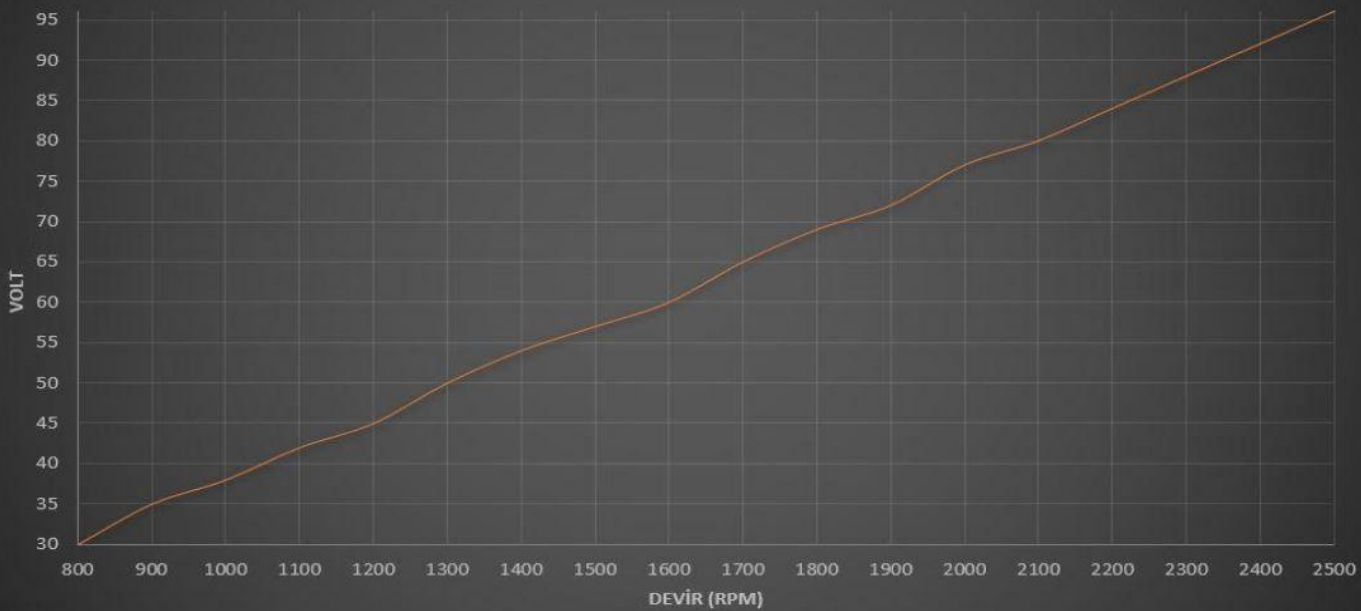
500G-24V-Generator-Rpm-Volt-Graphic
