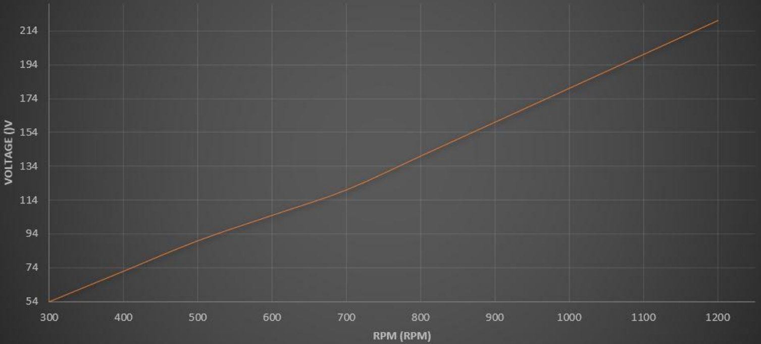
G-1500 48V Power Generator Rpm-Voltage Graphic
